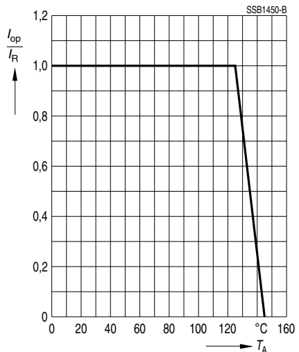
Current derating I_{\text{op}}/I_{\text{R}} versus ambient temperature T_{\text{A}}
