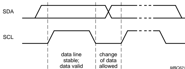
Fig.7 Bit transfer.
