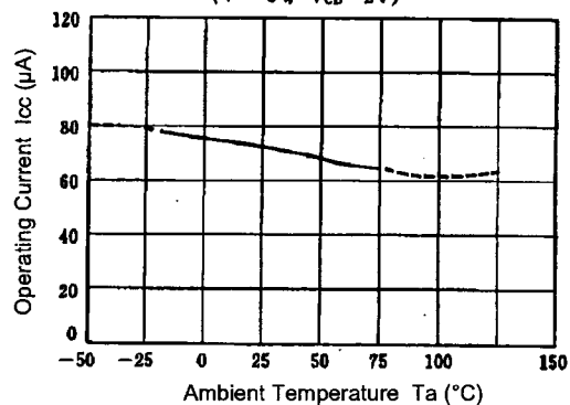
Operating Current vs. Ambient Temperature at Power Down Mode ( V^+=3\text{V} , V_{CD}=2\text{V} )
