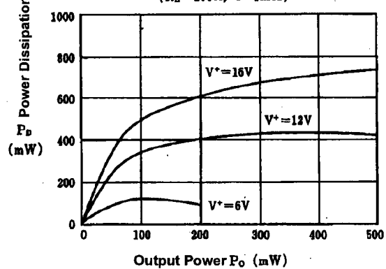
Power Dissipation vs. Output Power ( R_L=100\Omega , f=1\text{kHz} )
