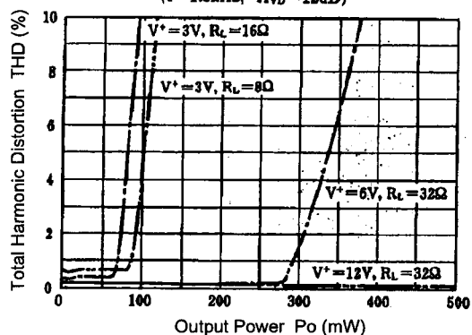
Total Harmonic Distortion vs. Output Power ( f=1.3\text{kHz} , A_{VD}=12\text{dB} )
