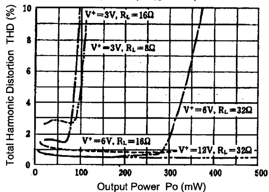
Total Harmonic Distortion vs. Output Power ( f=1\text{kHz} , A_{VD}=34\text{dB} )
