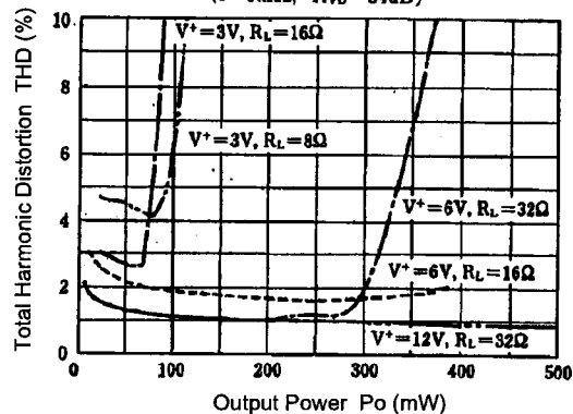
Total Harmonic Distortion vs. Output Power ( f=3\text{kHz} , A_{VD}=34\text{dB} )
